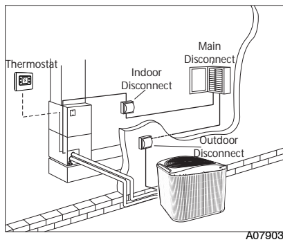
Fig. 2 - Electrical Disconnects
